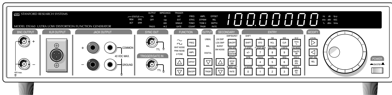
Figure 2-2 Front Panel
