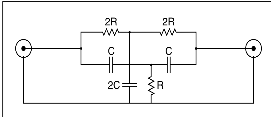
Figure 6-1 Twin-Tee Notch Filter
