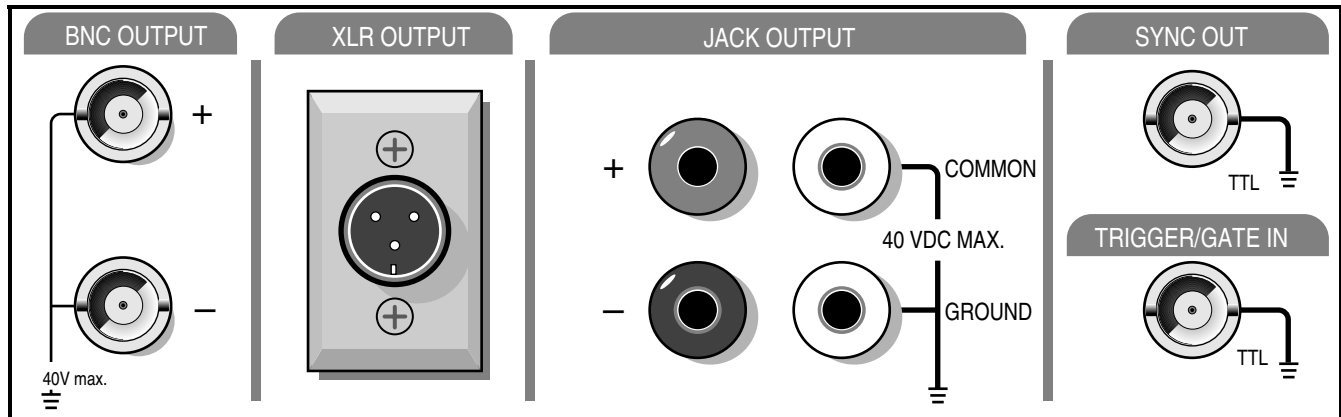
Figure 2-4 Outputs
